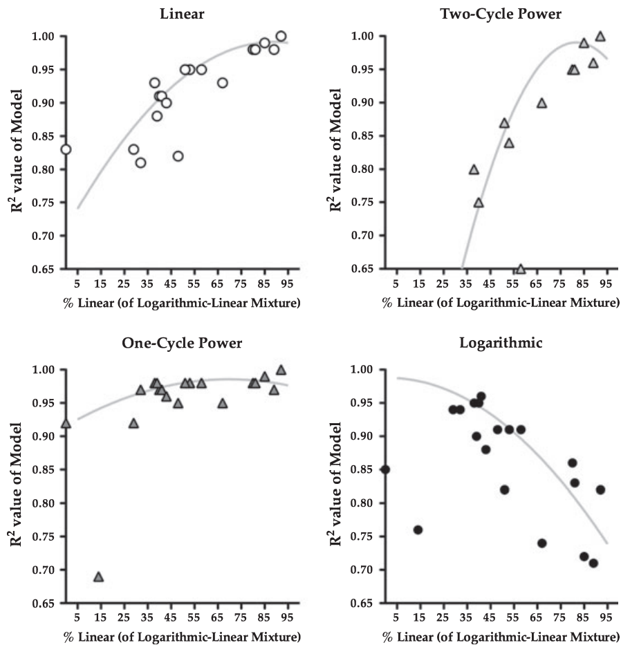
Figure 4 Linear, two-cycle model, one-cycle power and logarithmic models' fits to median estimates of 19 grade/study/range partitions, by the percentage of subjects in each study better fit by a linear than by a logarithmic model. Each of the four models' predicted fit, based on simulated mixtures of logarithmic and linear subjects, is shown in grey curves.
