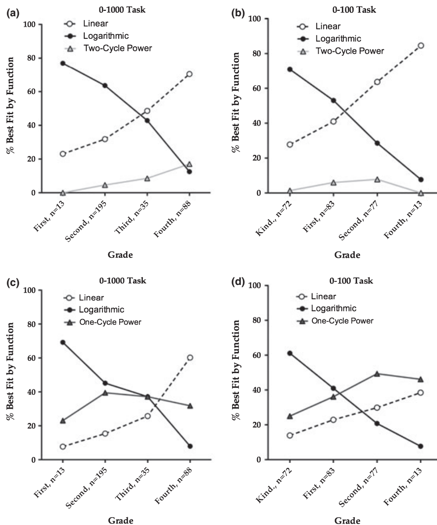
Figure 2 Percentages of individuals in eight studies fit by each function, separated by grade, range and models compared. Upper panels compare linear, logarithmic and two-cycle power models' fits separately for (a) 0–1000 range and (b) 0–100 range. Lower panels compare linear, logarithmic and one-cycle power model fits separately for (c) 0–1000 range and (d) 0–100 range.
