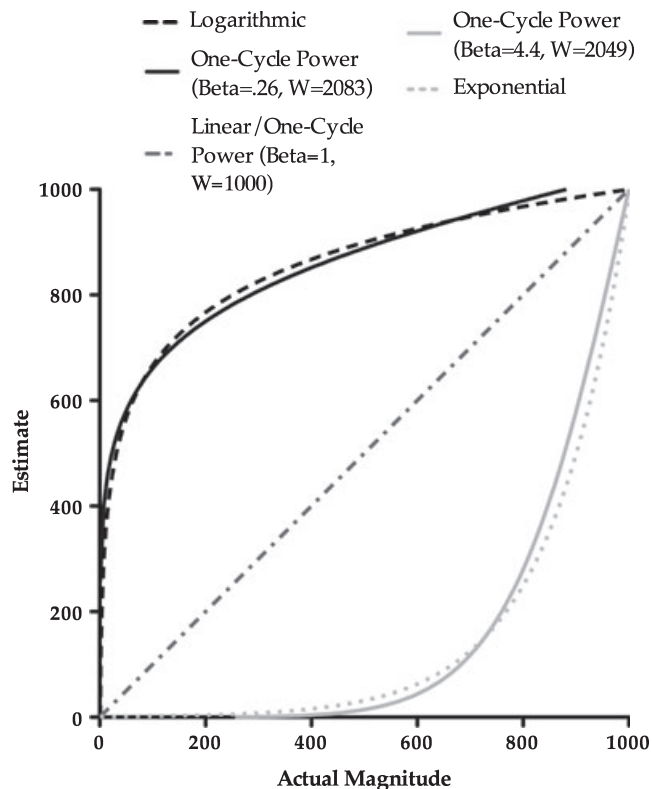
Figure 1 Estimates predicted by ideal logarithmic, linear, and exponential functions, and three one-cycle power models that most closely fit them.
