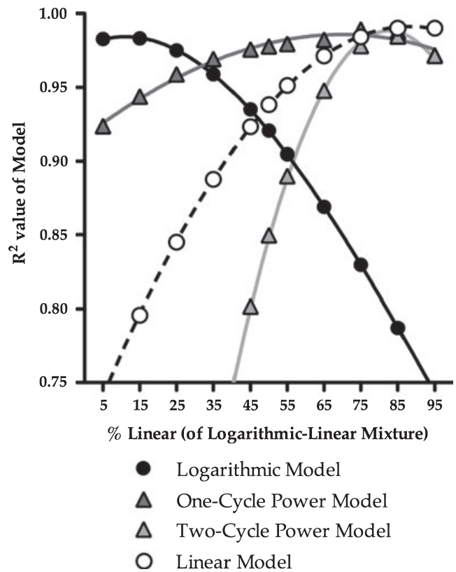
Figure 3 Logarithmic, one-cycle power, two-cycle power, and linear models' fits to data generated by mixing 100 simulated logarithmic and linear subjects.
